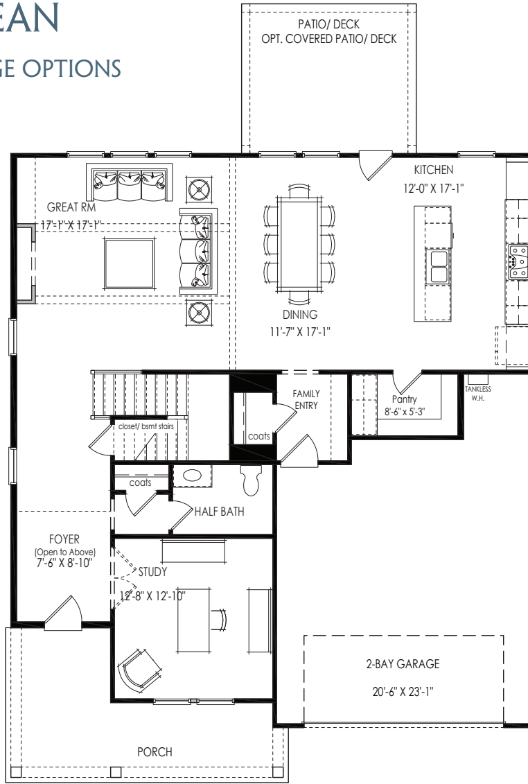
BASE PLAN
