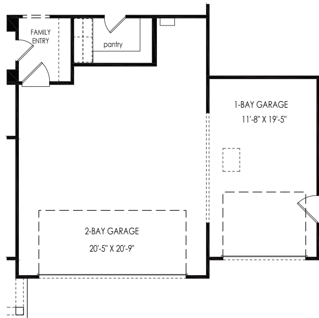
3-CAR GARAGE
